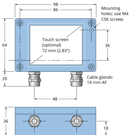
Electronics Module
