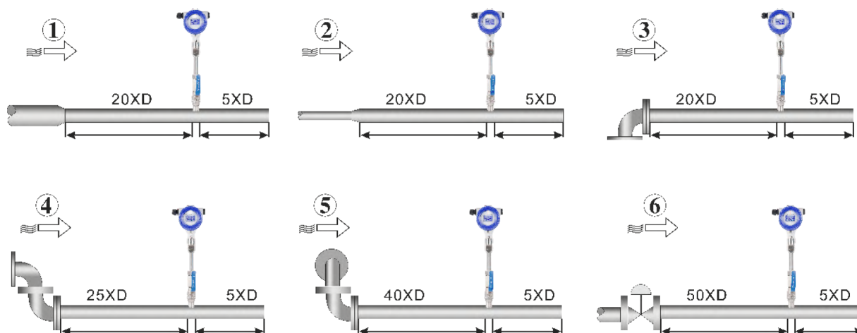
Installation upstream and downstream straight pipe
