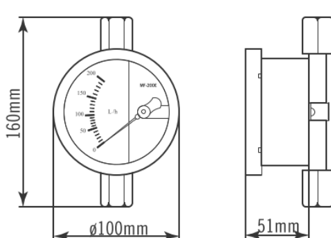
IP68 Model: MF200E-S
