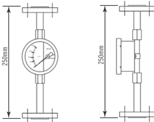
IP68 Model: MF200E-T
