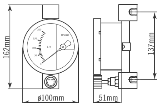
IP66 Model: MF200E-B
