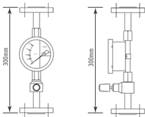
IP66 Model: MF200E-R
